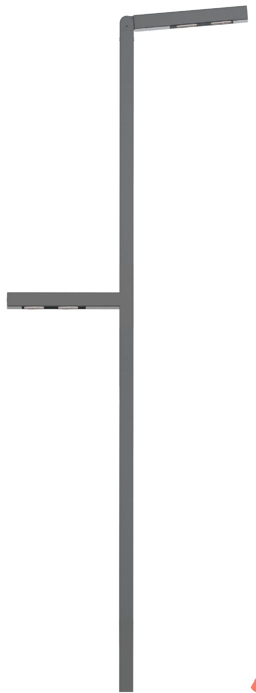
F | 22' 11/8" Pole 3' 11/4" Luminaire w/ 5° Tilt @ Top 3' 11/4" Luminaire w/ 0° Tilt @ 13' 1/2"
