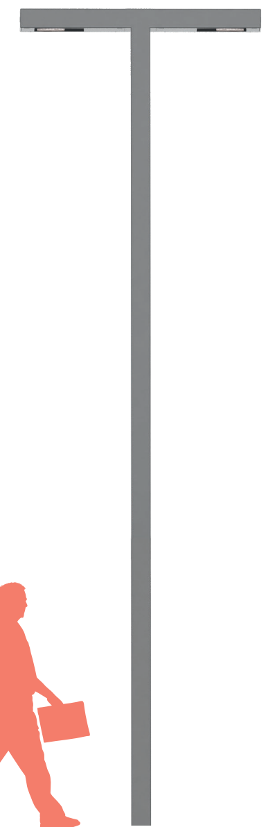
G | 19' 8/8" Pole (2) 3' 11/4" Luminaires w/ 0° Tilt @ Top
