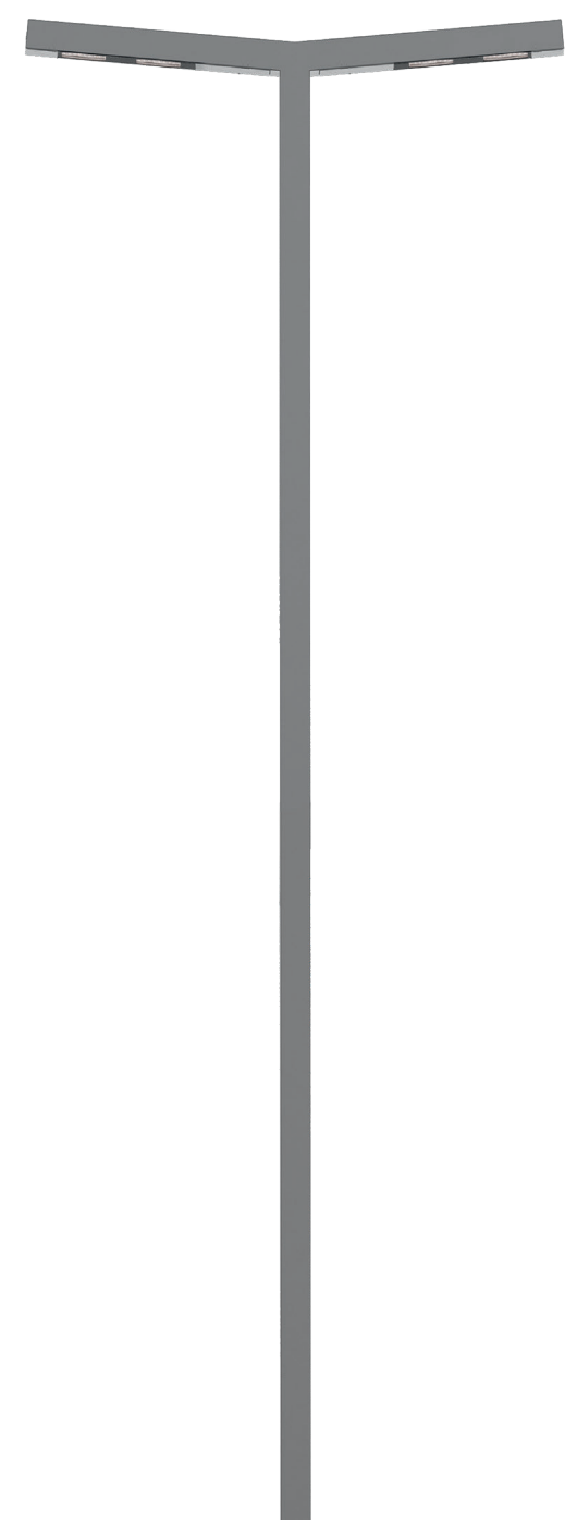
H | 22' 11/8" Pole (2) 3' 11/4" Luminaires w/ 5° Tilt @ Top
