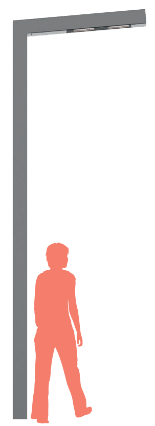
D | 13' 1/2" Pole 3' 11/4" Luminaire w/ 5° Tilt
